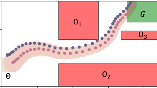
Fig. 1. The settings for controller synthesis of a mobile robot with reach-avoid specification.
