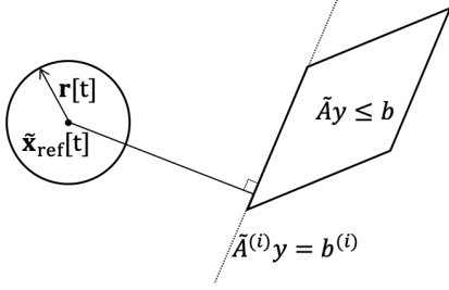
Fig. 2. Illustration of B_{\mathbf{r}[t]}(\tilde{\mathbf{x}}_{\text{ref}}[t]) being disjointed from the polytope \{y \mid \tilde{A}y \leq b\} .
